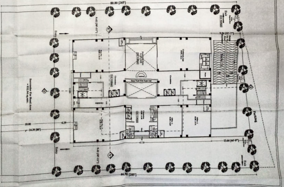
51.83 [170'] Ground Floor Plan (Commercial)
